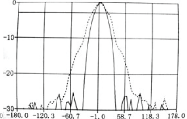
12000MHz(35° /26° )
